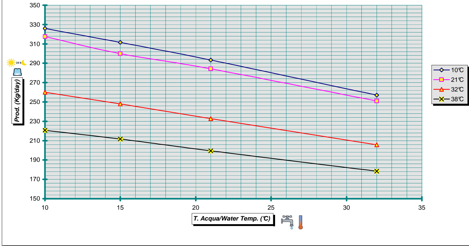
CM 650 (A/W) - Performances Data
